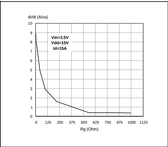
Figure 21. Turn-on current slope, V_{IN} = 3.5\text{ V}
