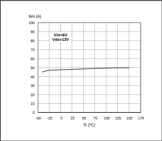
Figure 30. Derating curve
