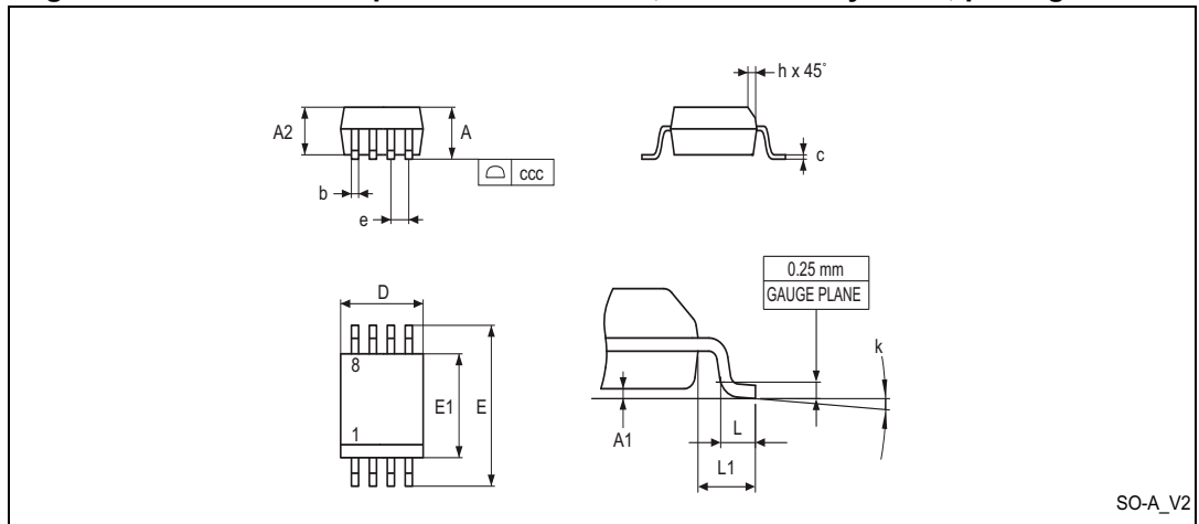
Figure 16. SO8N – 8-lead plastic small outline, 150 mils body width, package outline
