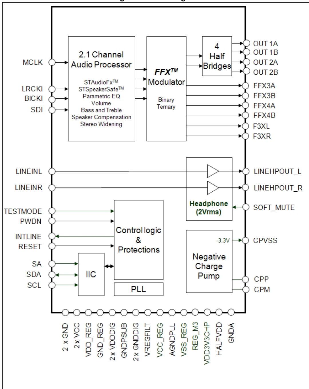
Figure 1. Block diagram
