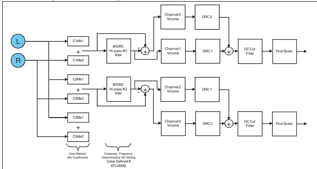
Figure 8. Processing path, second part: 2.0 output with B 2 DRC
