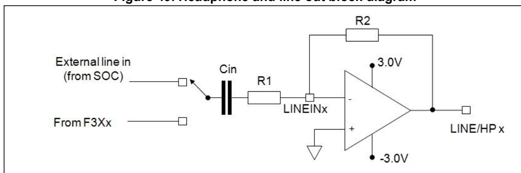
Figure 49. Headphone and line out block diagram
