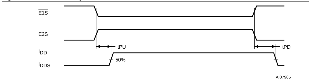
Figure 16. SRAM Standby AC Waveforms
