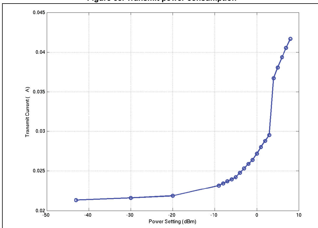
Figure 58. Transmit power consumption
