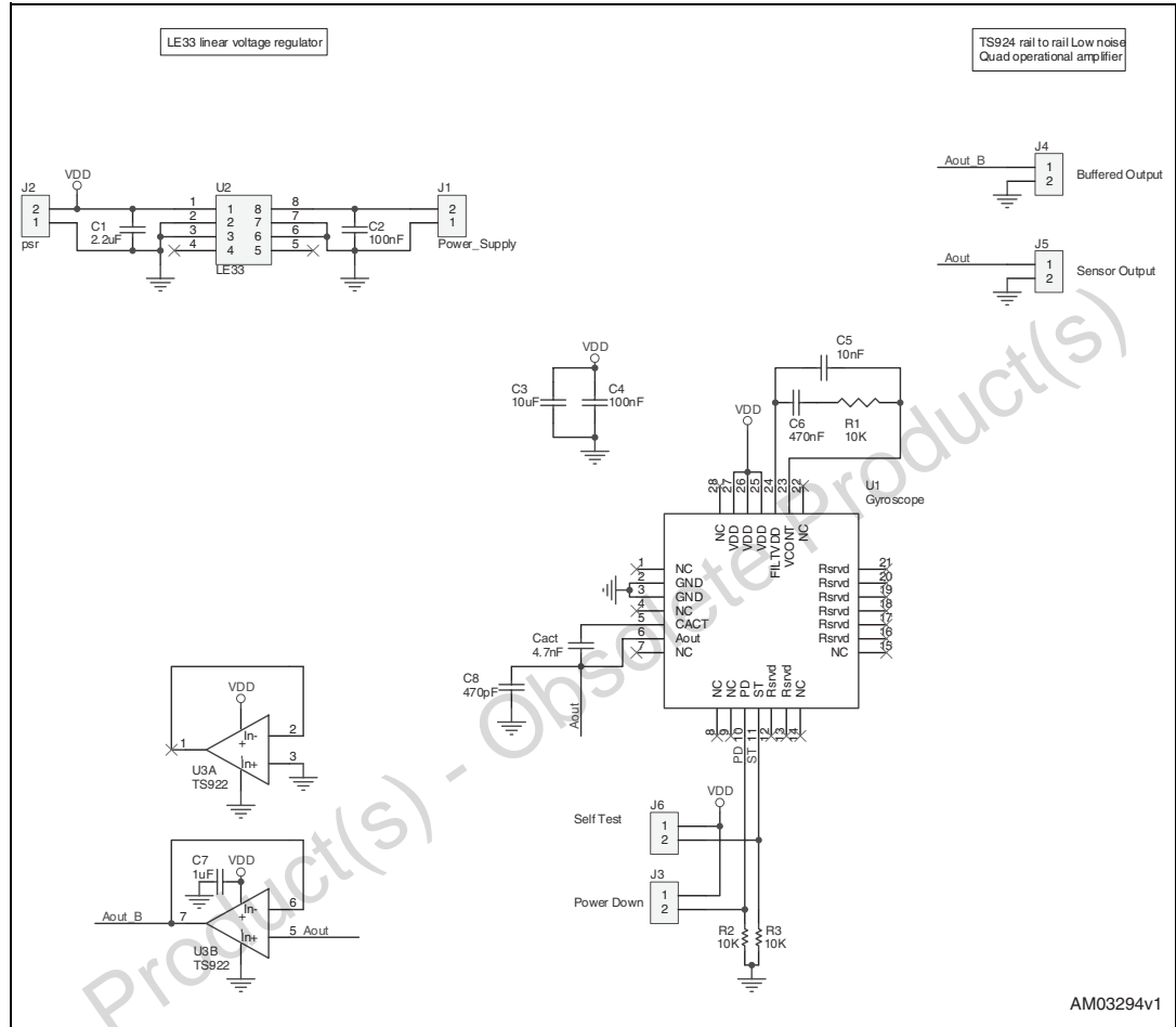
Figure 1. Circuit schematic
