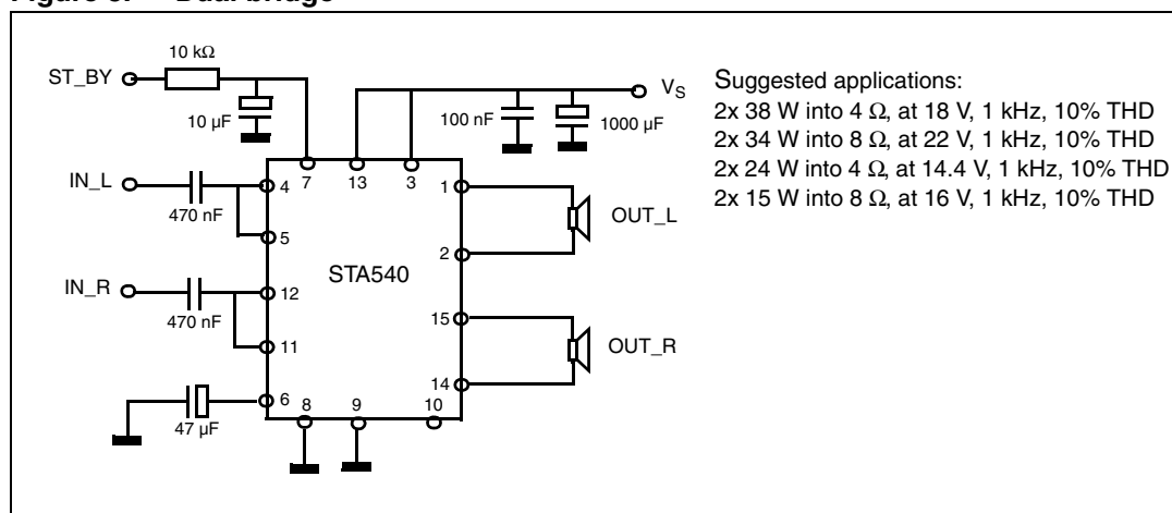
Figure 5. Dual bridge
