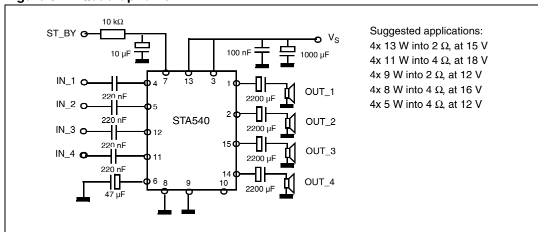
Figure 3. Quadraphonic
