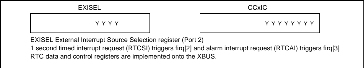
Figure 50 : ESFRs and Port Pins Associated with the RTC
