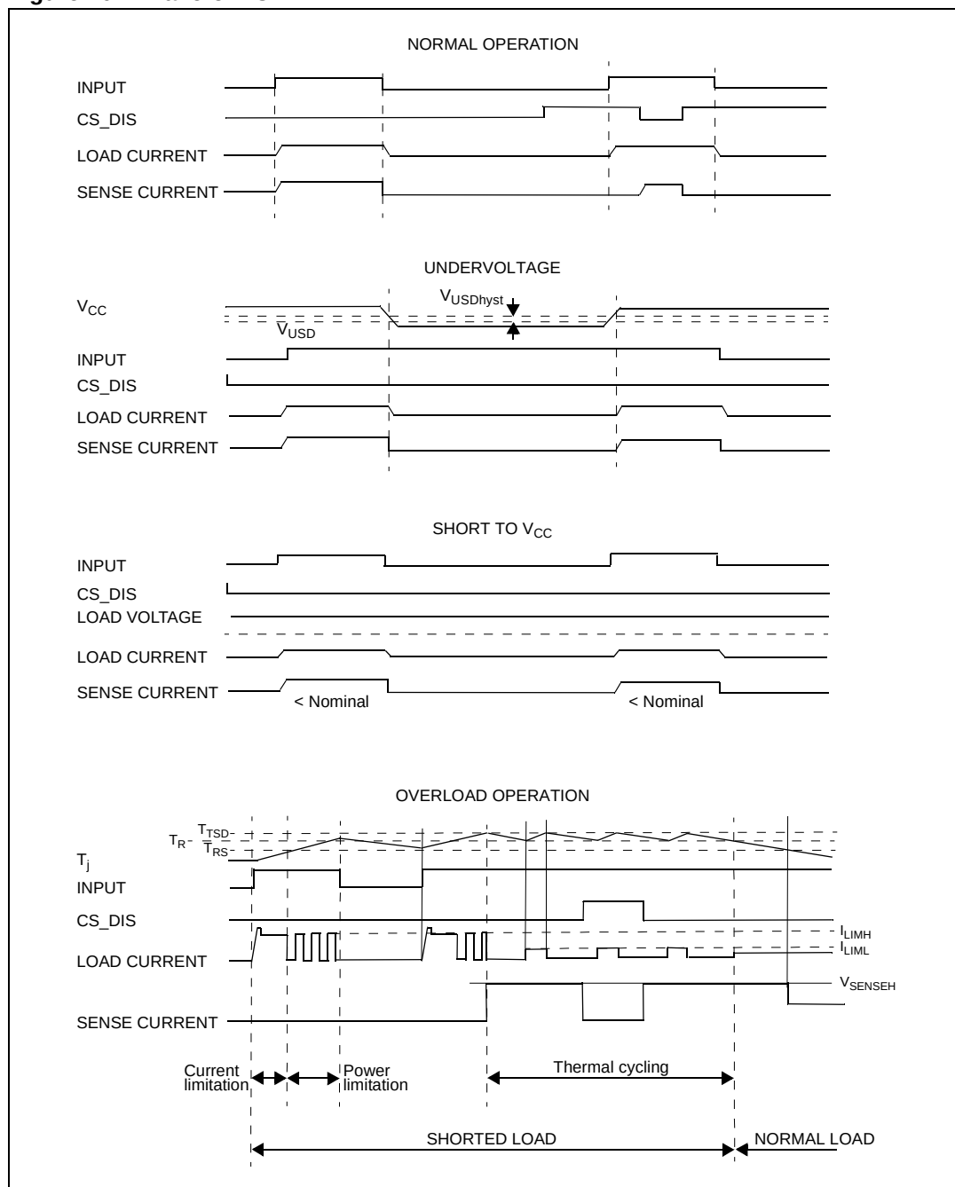
Figure 10. Waveforms
