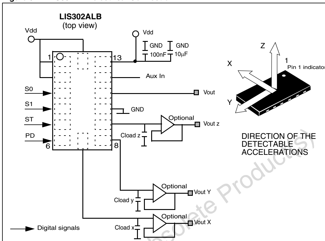
Figure 3. LIS302ALB electrical Connection
