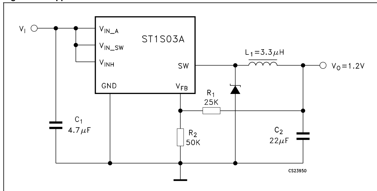
Figure 3. Application circuits
