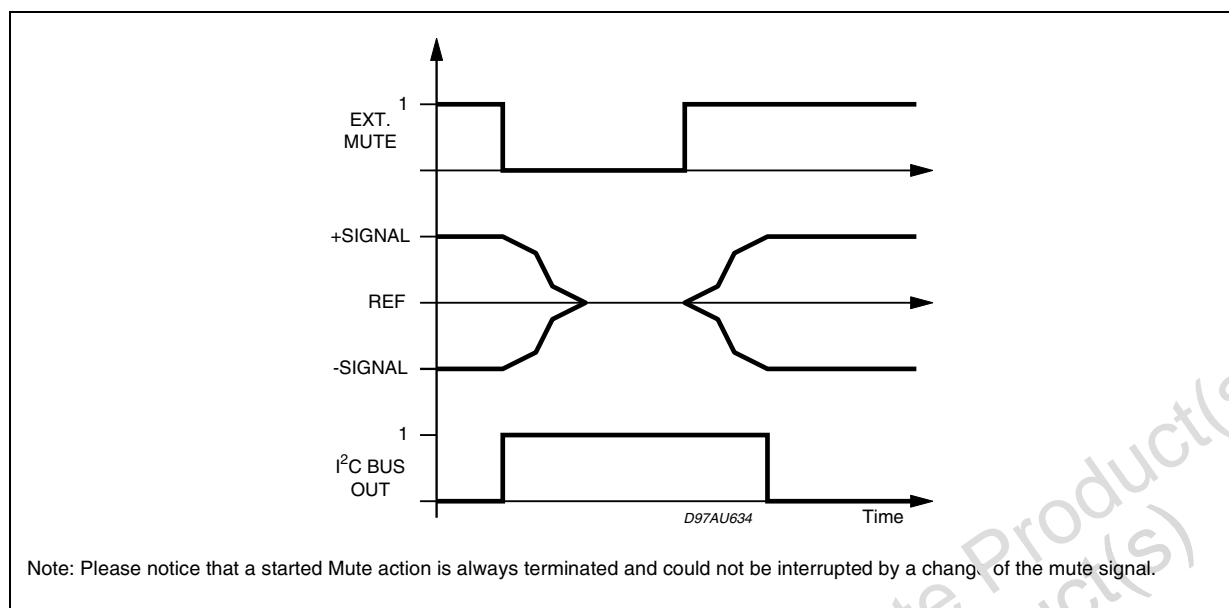
Figure 9. Softmute Timing
