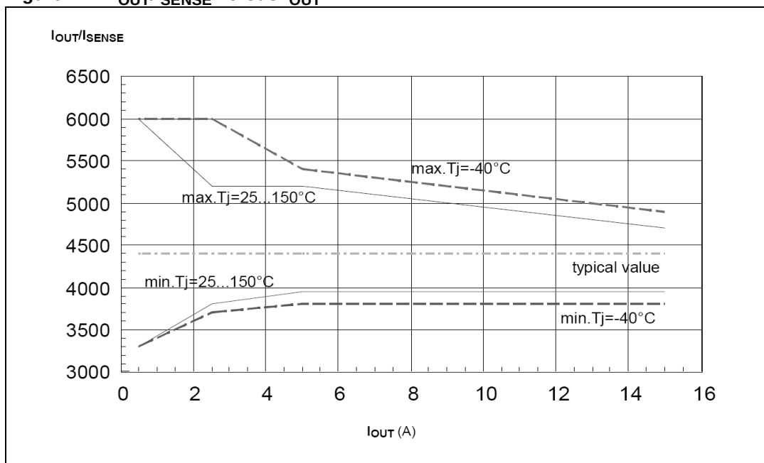
Figure 7. I_{OUT}/I_{SENSE} versus I_{OUT}
