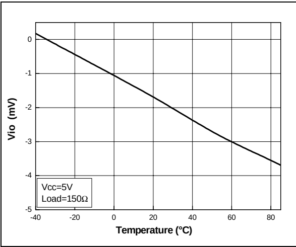
Figure 15. Input offset vs. temperature
