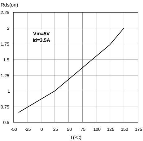
Figure 42. Normalized On Resistance Vs. Temperature
