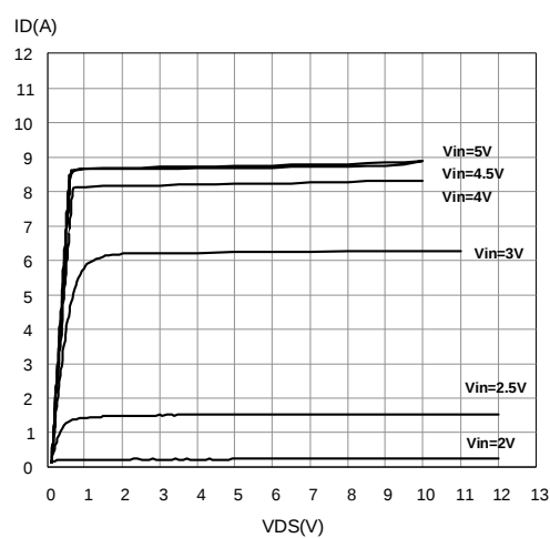
Figure 33. Output Characteristics
