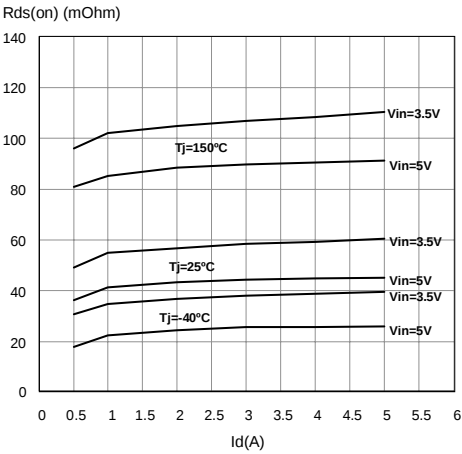
Figure 41. Static Drain-Source On resistance Vs. Input Voltage
