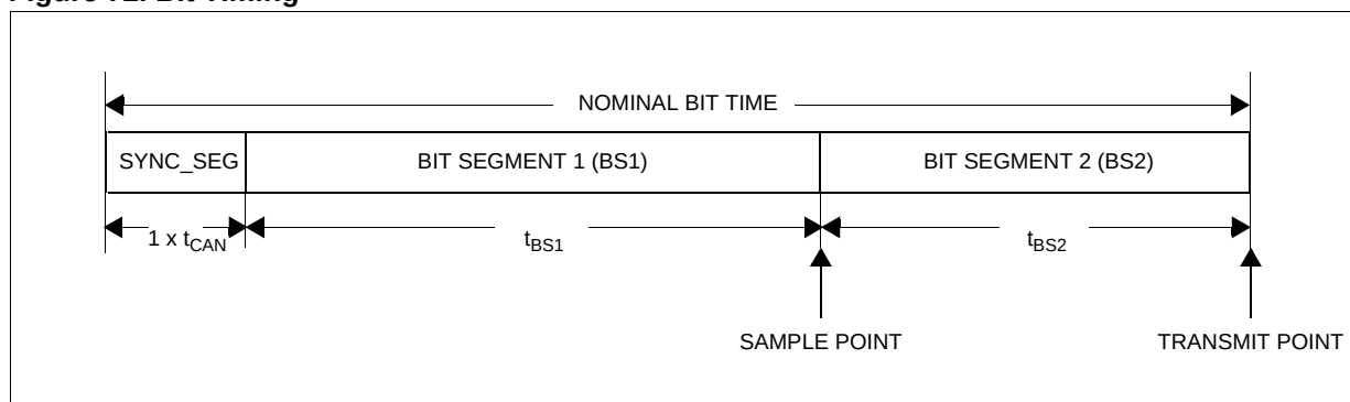
Figure 72. Bit Timing
