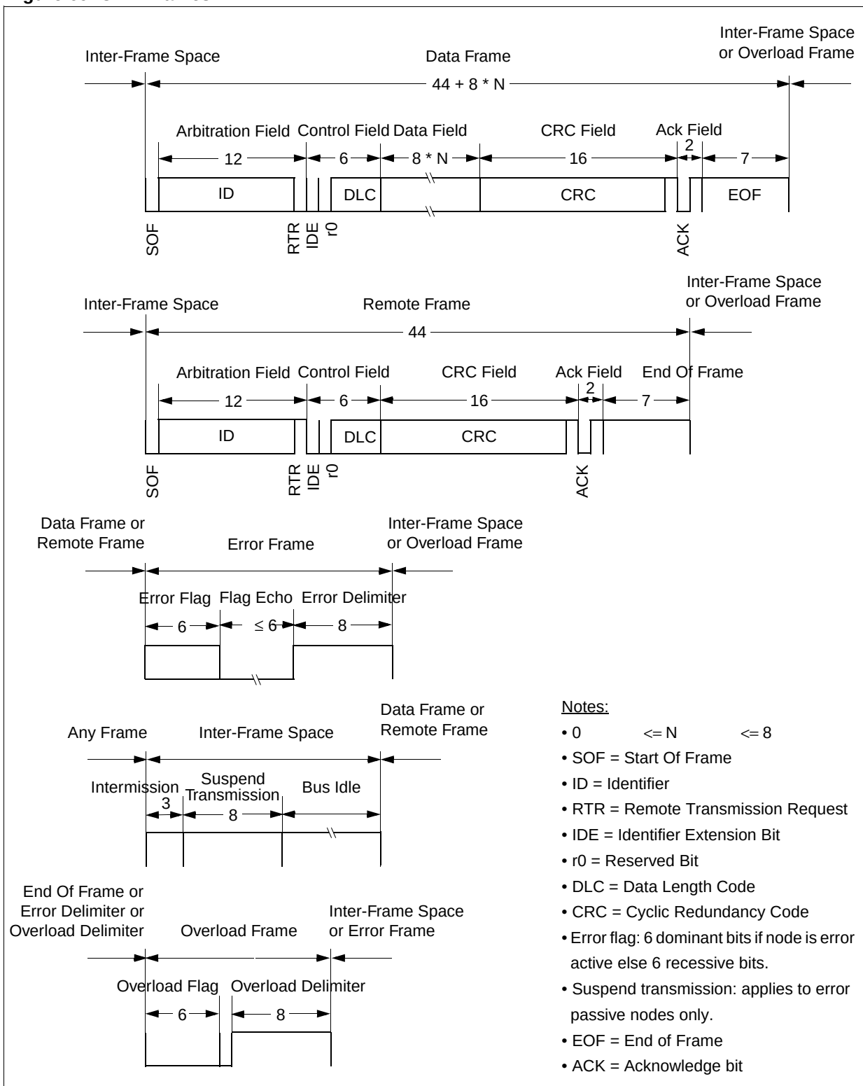
Figure 69. CAN Frames
