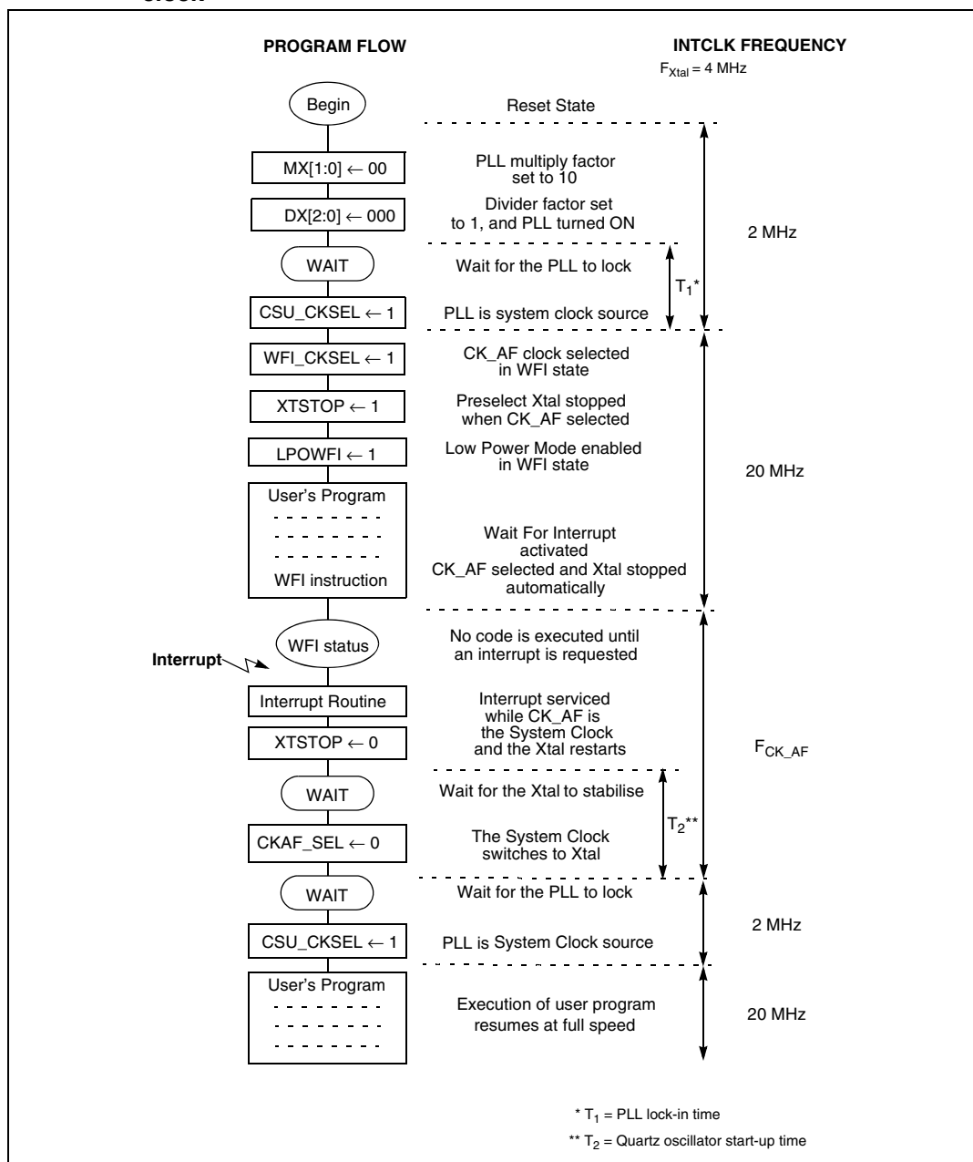
Figure 63. Example of low power mode programming in WFI using CK_AF external clock
