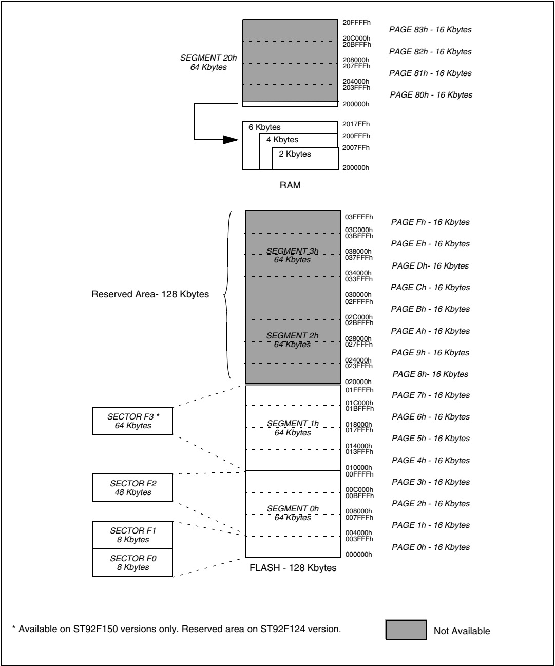
Figure 42. ST92F124/F150 internal memory map (128K versions)
