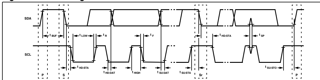
Figure 193. I 2 C timing
