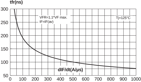
Fig. 9: Forward recovery time versus dI_F/dt (90% confidence).
