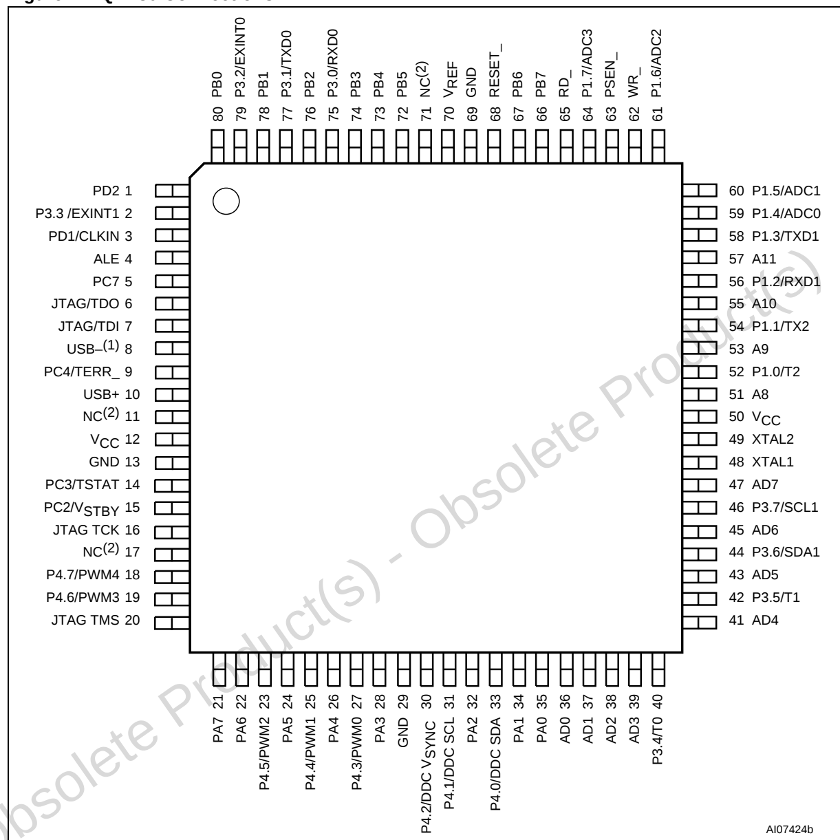
Figure 4. TQFP80 Connections
