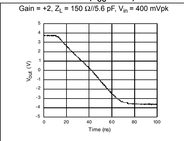
Figure 22. Large signal measurement - negative slew rate ( V_{CC} = \pm 5 V)
