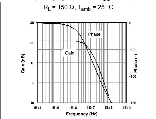
Figure 20. Closed loop gain and phase vs. frequency (gain = +11, V_{CC} = \pm 5 V)
