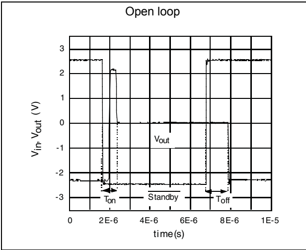
Figure 14. Standby mode - T_{on} , T_{off} ( V_{CC} = \pm 2.5 V)
