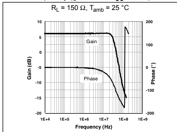
Figure 17. Closed loop gain and phase vs. frequency (gain = +2, V_{CC} = \pm 5 V)
