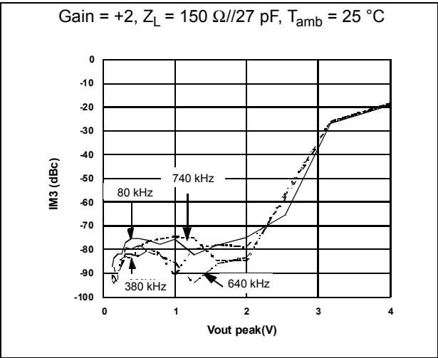
Figure 15. Third order intermodulation ( V_{CC} = \pm 2.5 V) (1)
