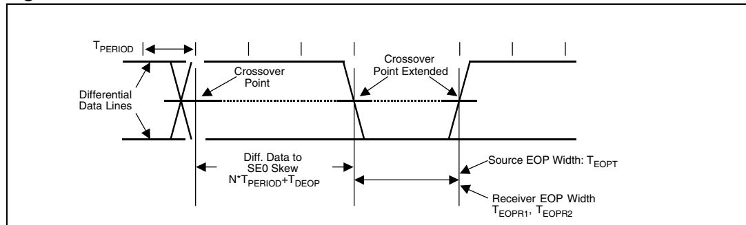
Figure 43. Differential to EOP transition skew and EOP width
