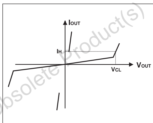
Fig. 2: ACS302 switch static characteristic.
