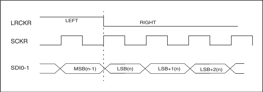
Figure 7. SAI protocol (when: RLRS=1; RREL=0; RCKP=1; RDIR=1)
