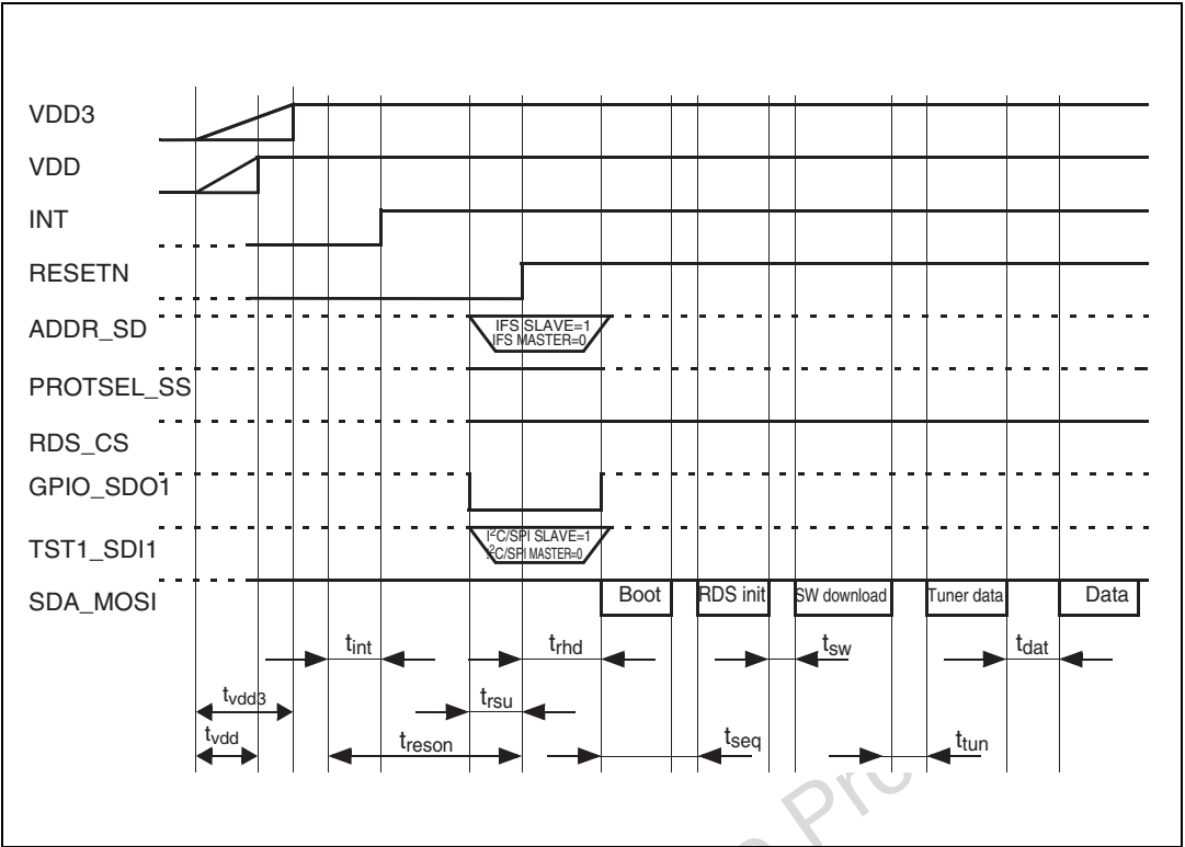
Figure 3. Power on and boot sequence using I 2 C
