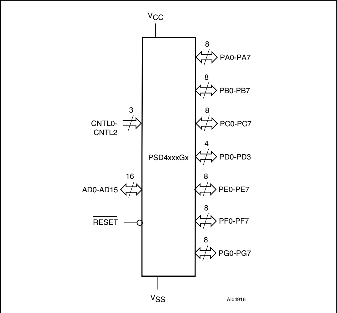
Figure 1. Logic diagram
