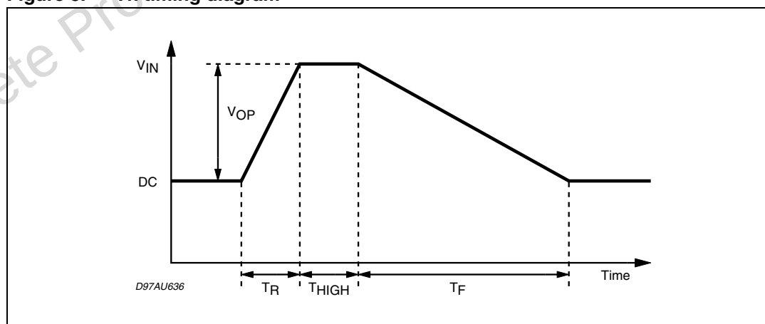
Figure 3. Vn timing diagram
