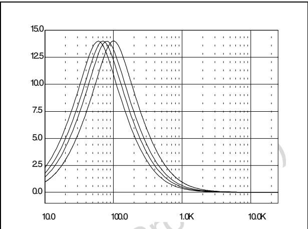
Figure 12. Bass normal and DC mode @ Gain = 14dB, f_c = 80\text{Hz}
