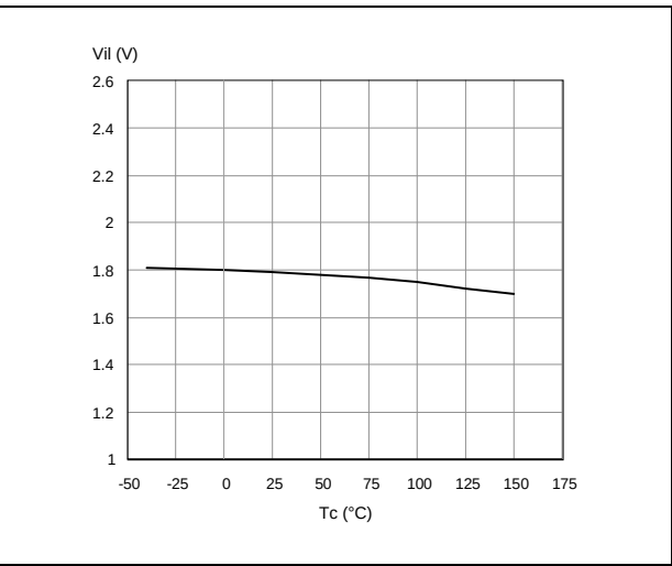
Figure 18. Input low-level
