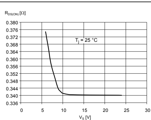
Figure 35. Typical high-side R_{DS(ON)} vs. supply voltage
