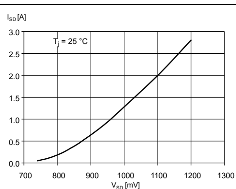
Figure 39. Typical drain-source diode forward ON characteristic
