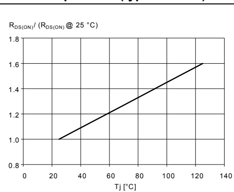
Figure 37. Normalized R_{DS(ON)} vs. junction temperature (typical value)
