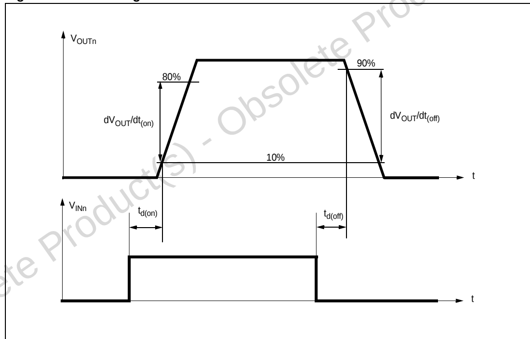
Figure 5. Switching characteristics
