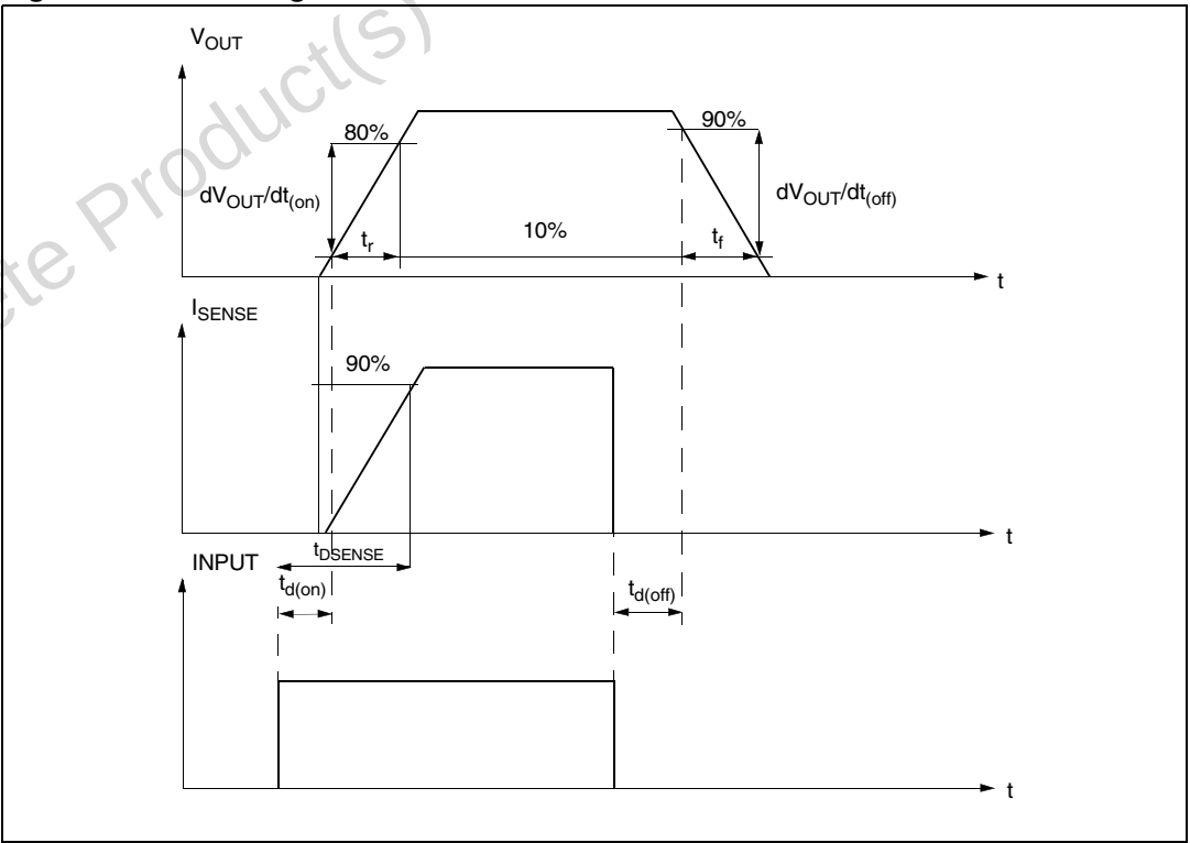
Figure 5. Switching characteristics
