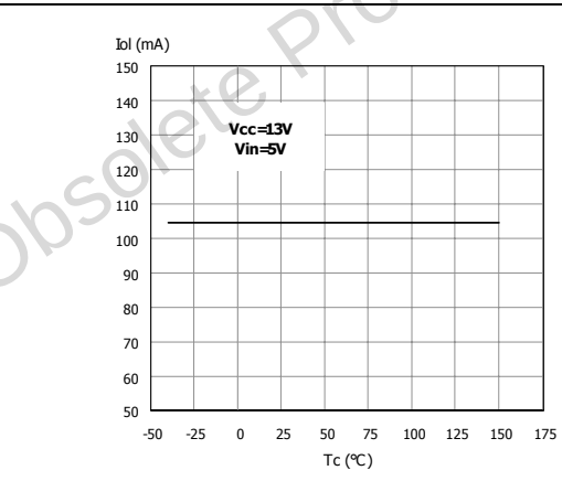
Figure 22. Open load on-state detection threshold
