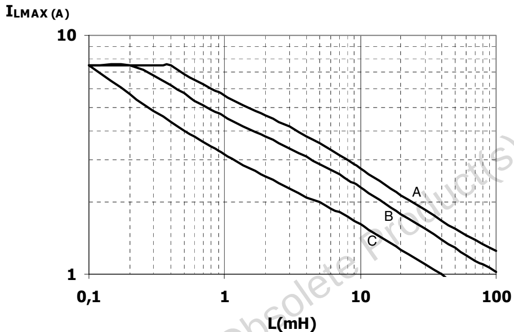
Figure 26. Maximum turn-off current versus load inductance
