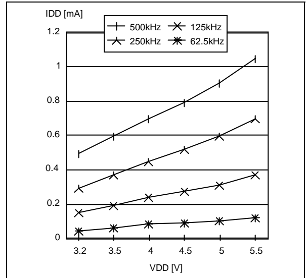
Figure 64. Typical I_{DD} in SLOW vs. f_{CPU}
