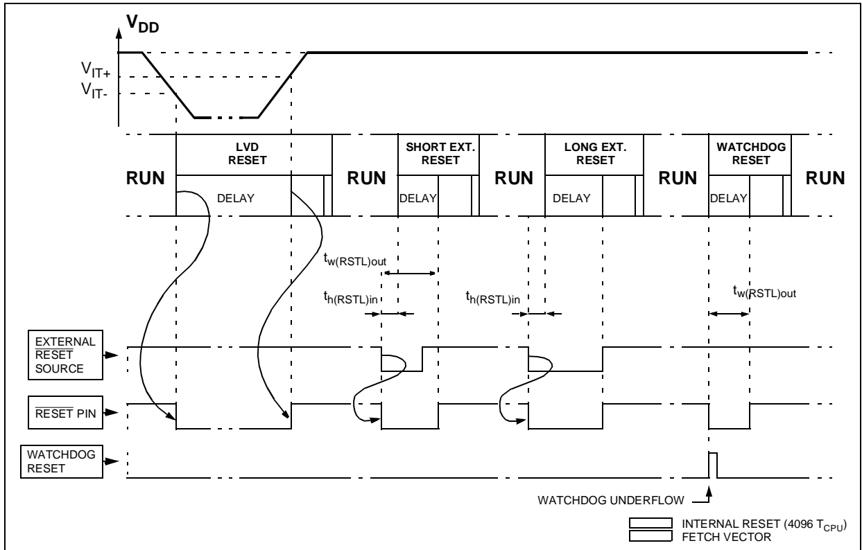
Figure 16. RESET Sequences
