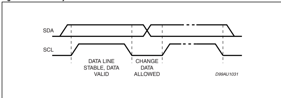
Figure 2. Data Validity on the I 2 C BUS
