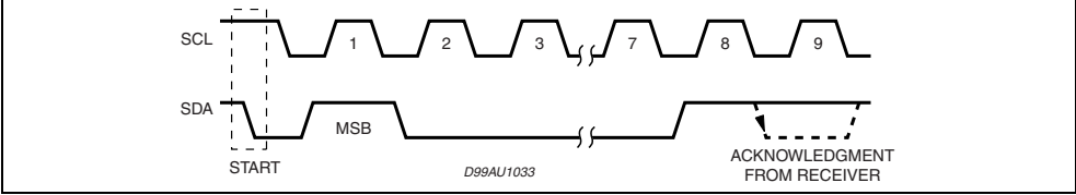
Figure 4. Acknowledge on the I 2 C BUS
