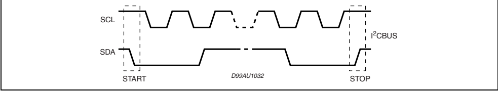
Figure 3. Timing Diagram on the I 2 C BUS
