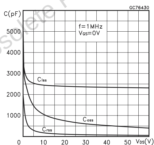
Figure 10. Capacitance Variations
