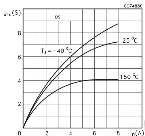
Figure 9. Transconductance
