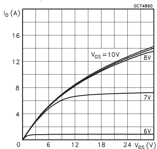
Figure 7. Output Characteristics
