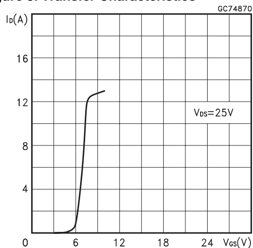
Figure 8. Transfer Characteristics
