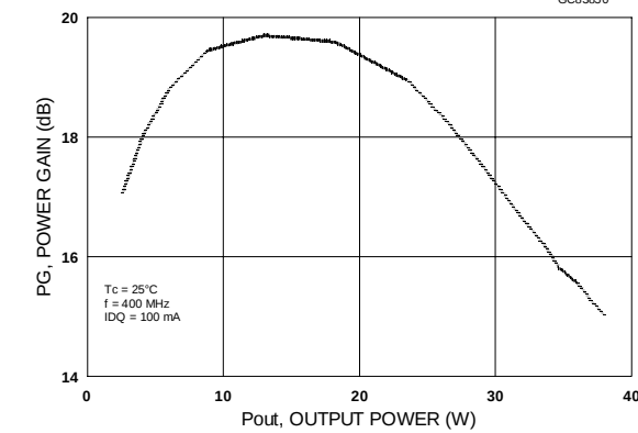
Power Gain vs Output Power
