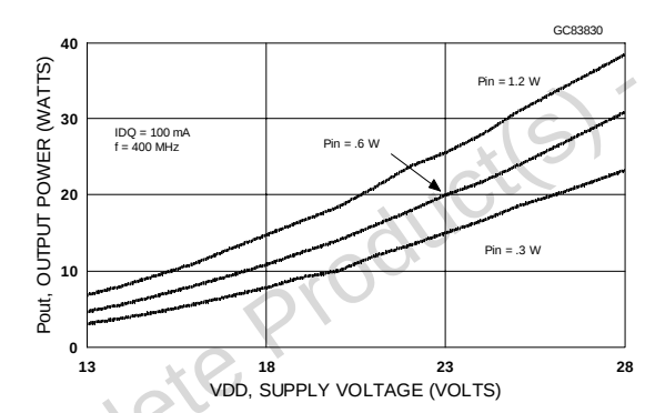
Output Power vs Voltage Supply
