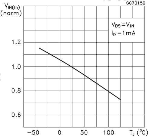
Figure 12. Normalized Input Threshold Voltage vs Temperature
