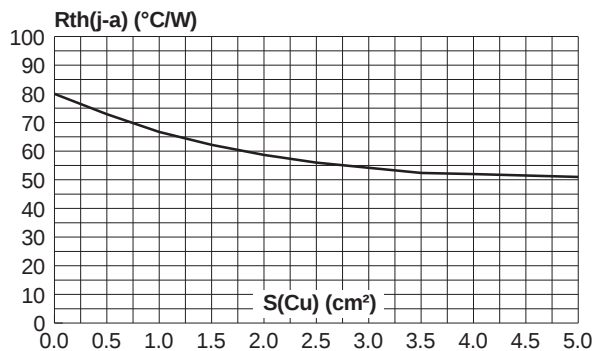
Fig. 11-1: Thermal resistance junction to ambient versus copper surface under each lead (Epoxy printed circuit board FR4, copper thickness: 35mm) (SMBYW04-200).
