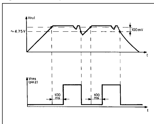
Figure 3. Reset Operation
