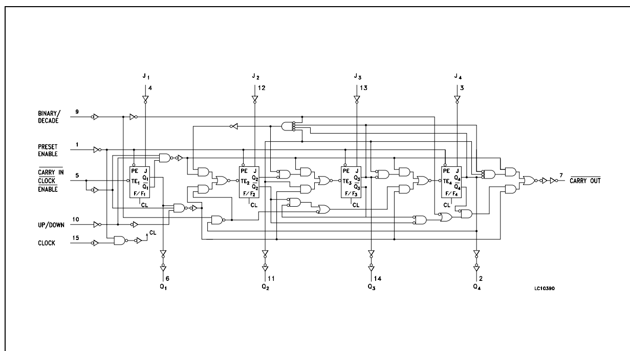
LOGIC DIAGRAM
