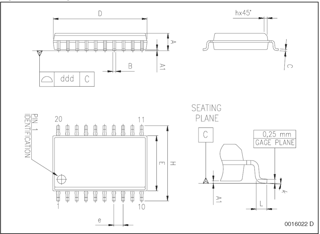
Figure 46. Package dimensions
