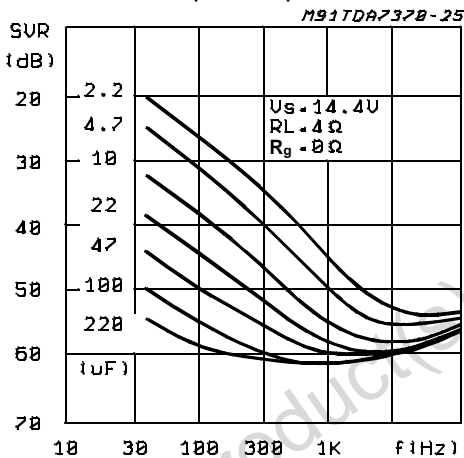
Figure 10: Supply Voltage Rejection vs. Frequency (Bridge) for different values of pin 6 capacitor.
