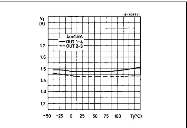
Figure 17. Free-wheeling diode forward voltage versus junction temperature at I_f = 1 A
