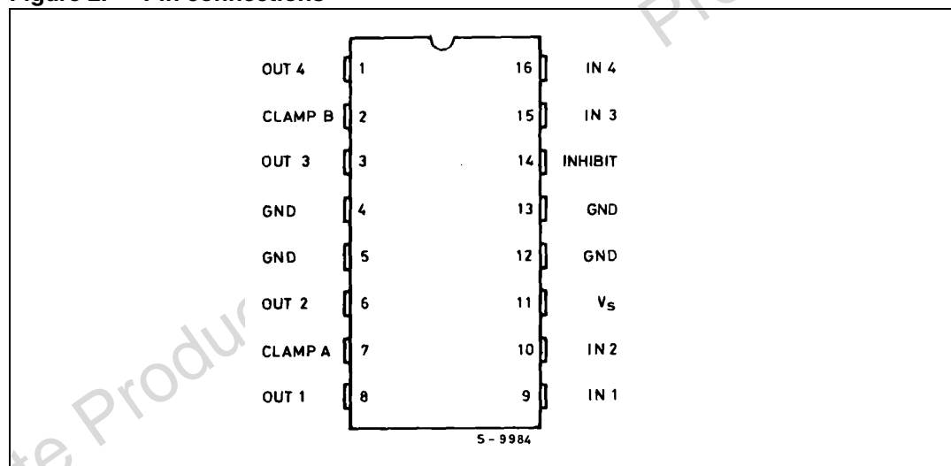
Figure 2. Pin connections
