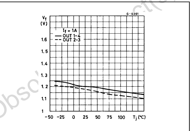
Figure 15. Free-wheeling diode forward voltage versus junction temperature at I_f = 1 A
