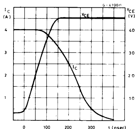
Figure 6. Turn-off Phase.
