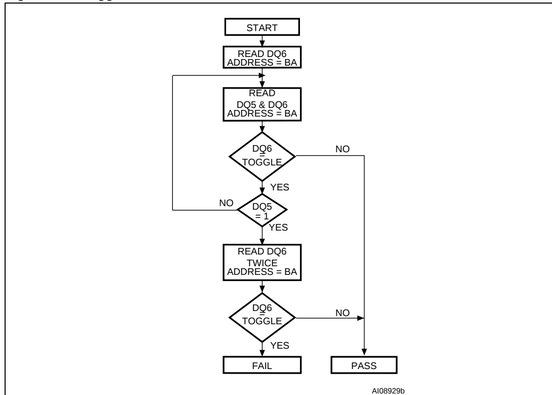
Figure 7. Toggle flowchart
