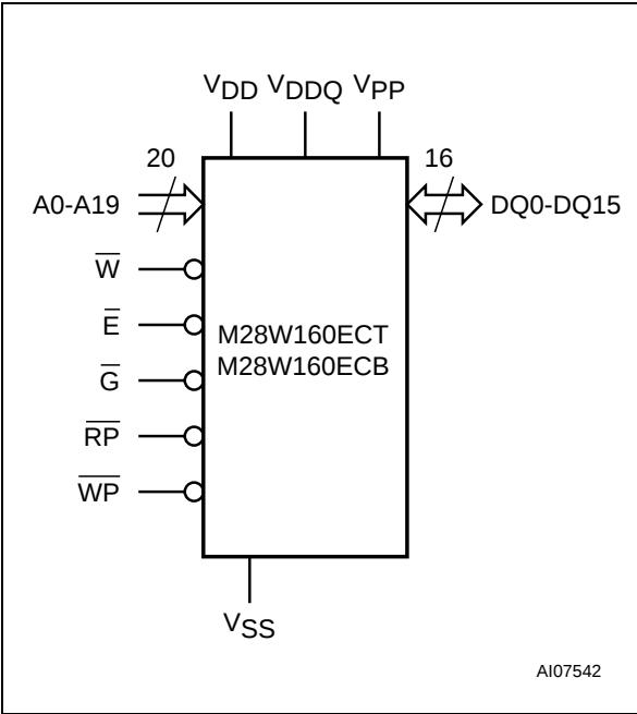
Figure 2. Logic Diagram
