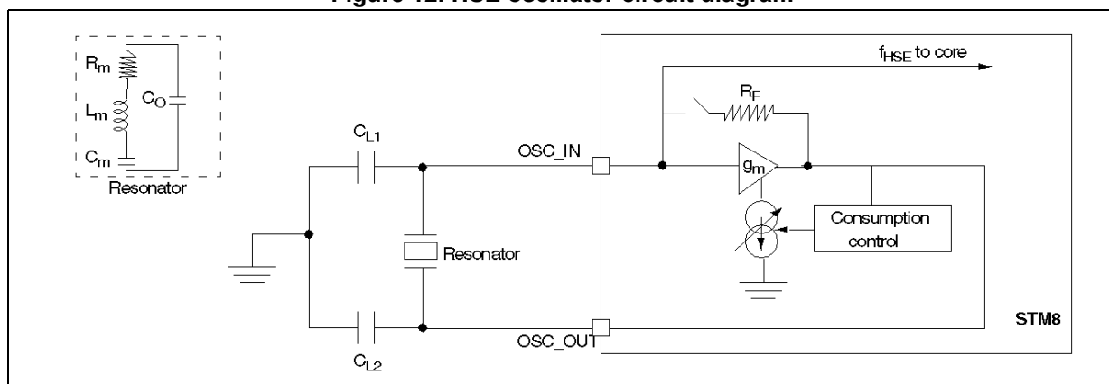
Figure 12. HSE oscillator circuit diagram
