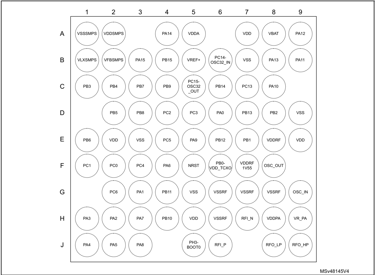
Figure 10. UFBGA73 pinout
