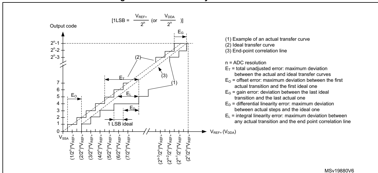
Figure 22. ADC accuracy characteristics
