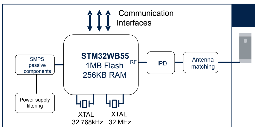
Figure 1. STM32WB5MMG module block diagram
