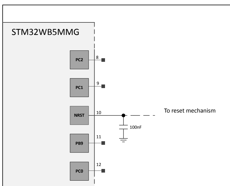
Figure 3. Reset circuit
