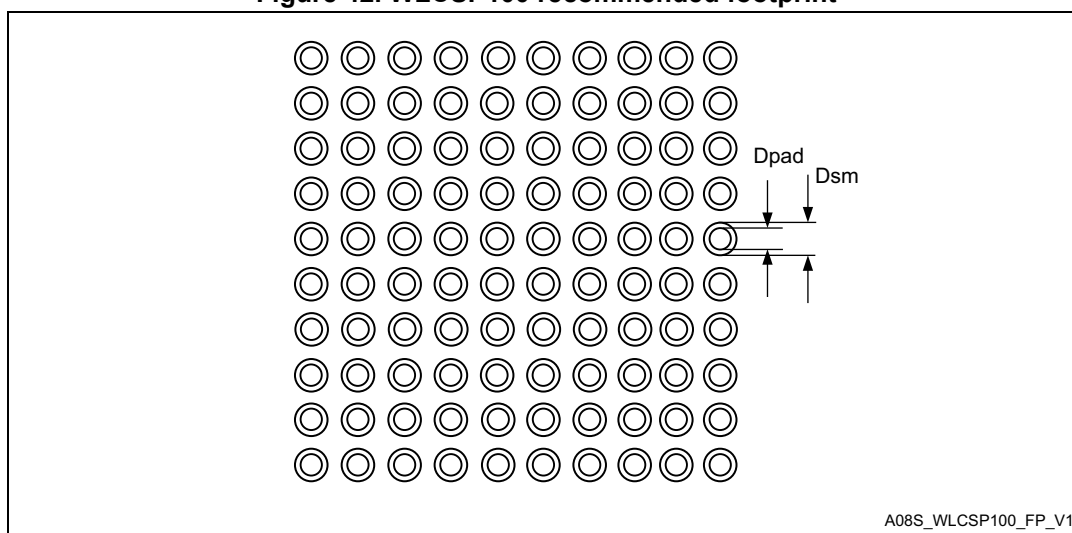
Figure 42. WLCSP100 recommended footprint
