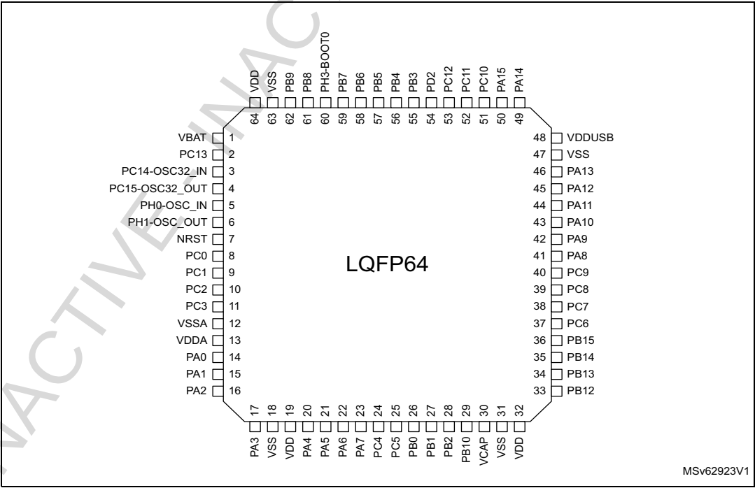
Figure 12. LQFP64 pinout
