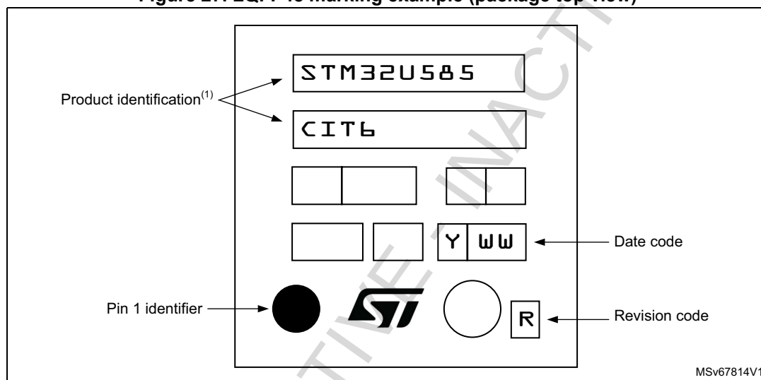
Figure 27. LQFP48 marking example (package top view)
