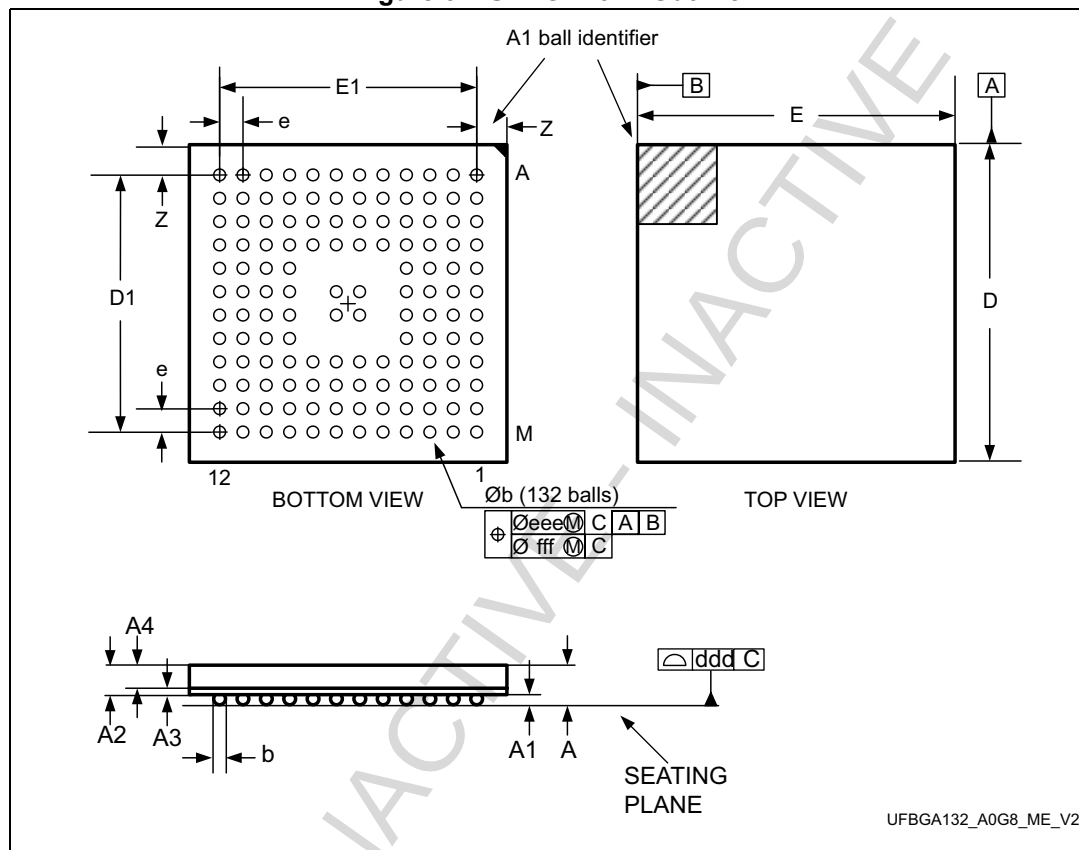
Figure 37. UFBGA132 - Outline
