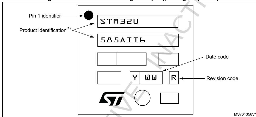
Figure 45. UFBGA169 marking example (package top view)
