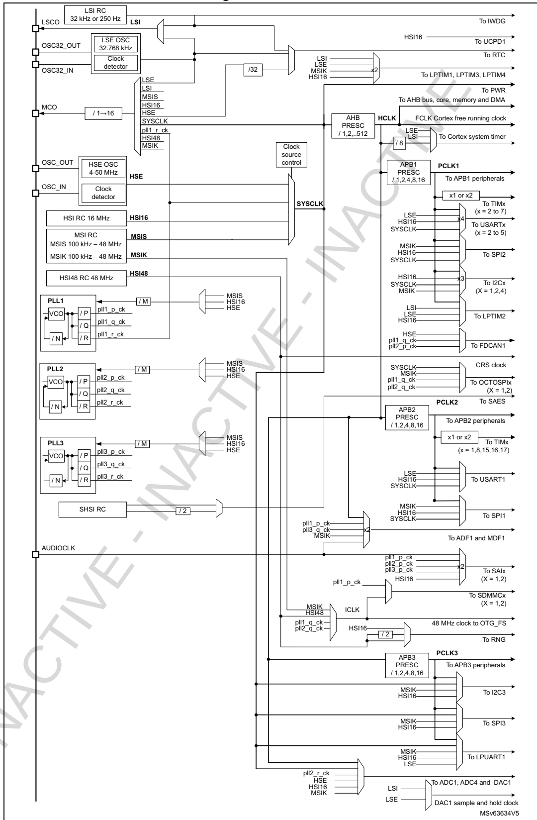
Figure 5. Clock tree
